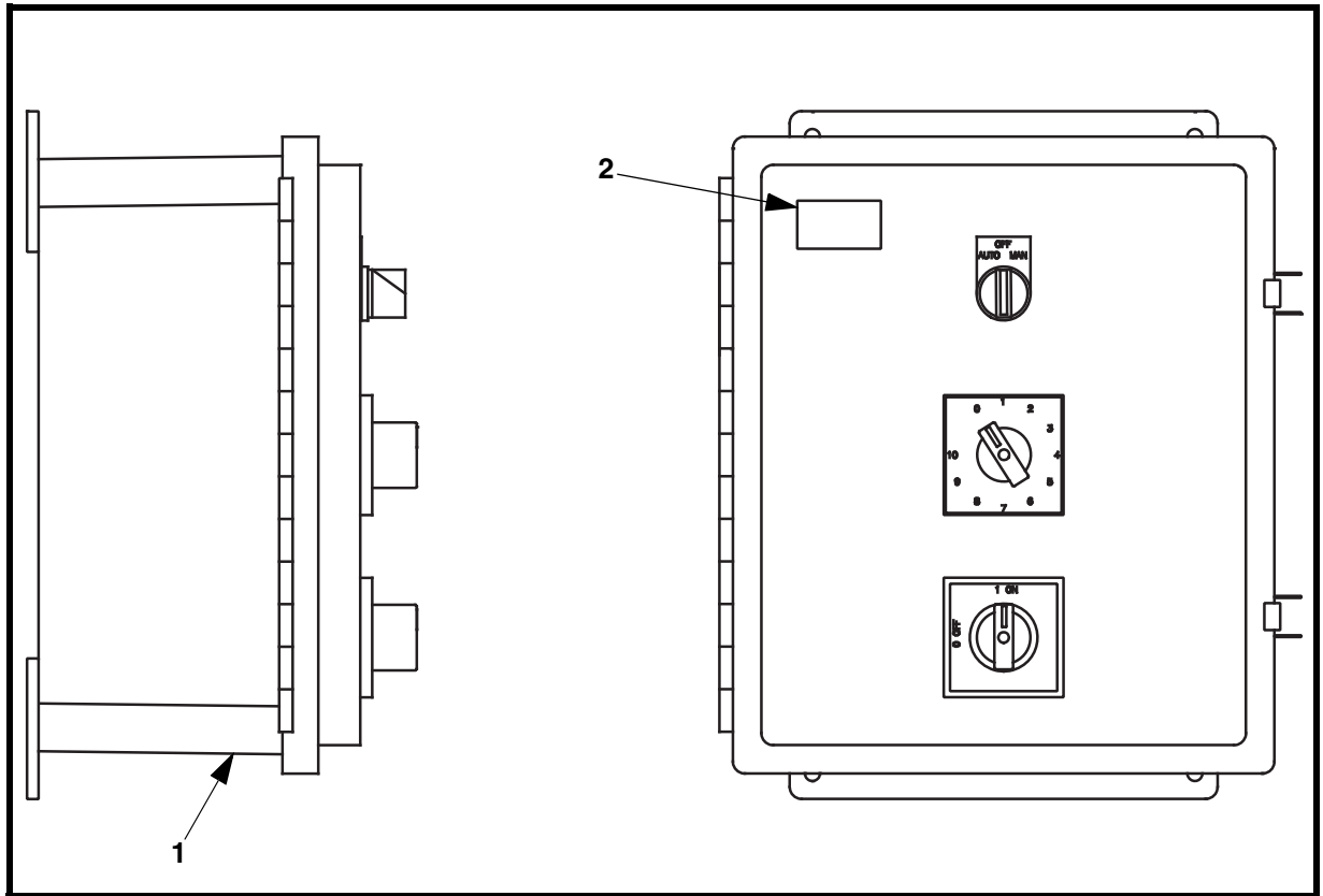
Figure 10. MARTIN® Sonic Horn Controller, P/N 38901-S
