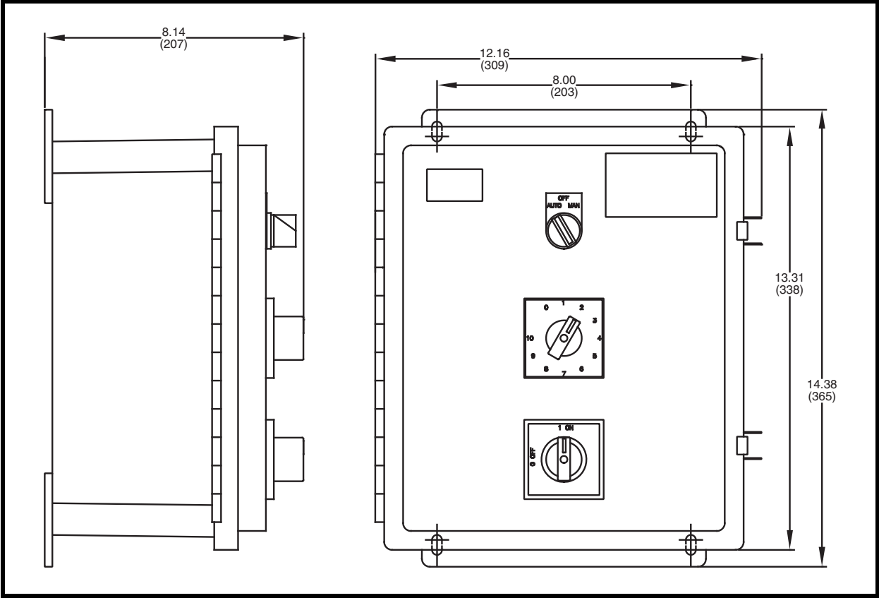
Figure 11. MARTIN® Sonic Horn Controller Dimensions
